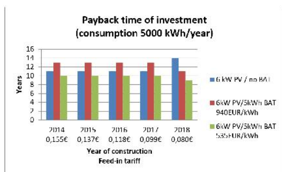
Figure 9: Payback of the investment in years of a 6 kW PV system with a 5 kWh battery pack with an annual electricity consumption of 5000 kWh/year.
